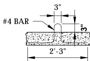
TYPICAL LIFT HOOP SECTION
