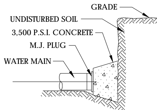
(ELEV. VIEW)
