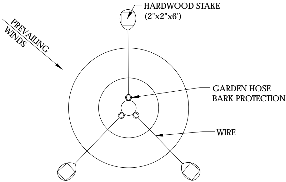
TREE GUYING & STAKING DETAIL
