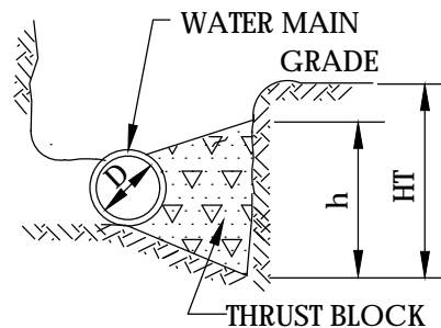
(ELEV. VIEW)
