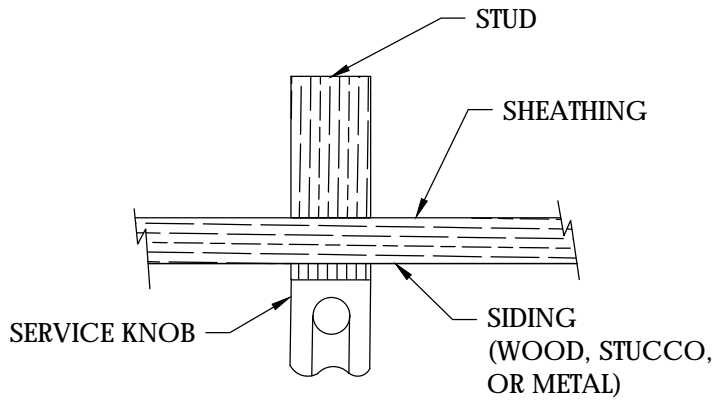
WOOD FRAME CONSTRUCTION
