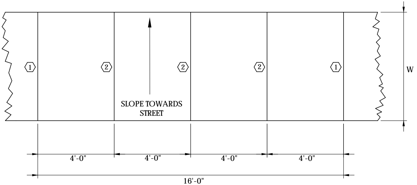
PLAN
