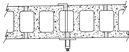
BRICK, CONCRETE, OR CINDER BLOCK
